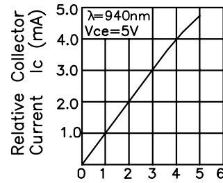
E_e —irradiance—mW/cm 2 IRRADIANCE VS. RELATIVE COLLECTOR CURRENT
