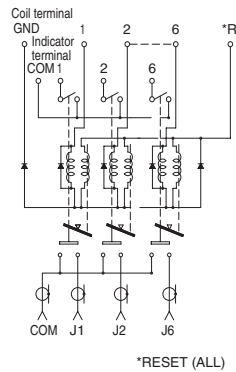
Latching type
