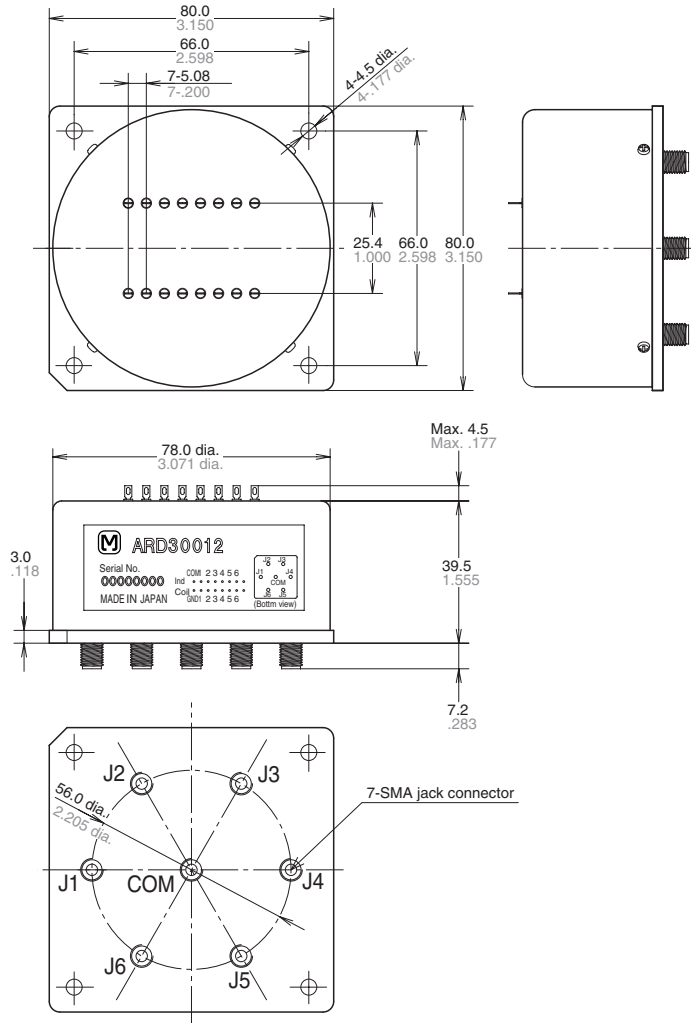
Latching type
