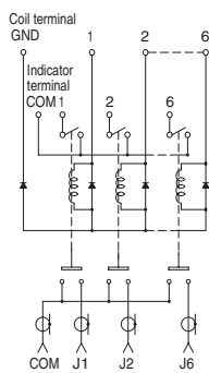
Fail-safe type
