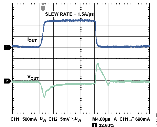
Figure 34. Load Transient Response, I_{\text{LOAD}} = 100\text{ mA} to 1.2 A, V_{\text{OUT}} = 3.3\text{ V} , V_{\text{IN}} = 4.0\text{ V} , C_{\text{OUT}} = 22\mu\text{F} , Channel 1 = I_{\text{OUT}} , Channel 2 = V_{\text{OUT}}
