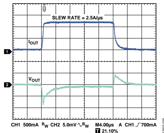
Figure 33. Load Transient Response, I_{\text{LOAD}} = 100\text{ mA} to 1.2 A, V_{\text{OUT}} = 3.3\text{ V} , V_{\text{IN}} = 4.0\text{ V} , Channel 1 = I_{\text{OUT}} , Channel 2 = V_{\text{OUT}}
