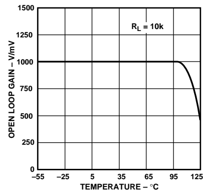
Figure 9. Open Loop Gain vs. Temperature
