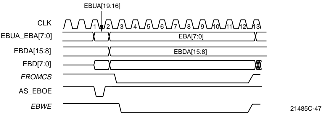
Figure 44. Flash Write from Expansion Bus Data Port
