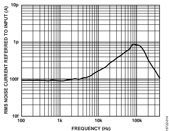
Figure 10. Noise Bandwidth/Peaking
