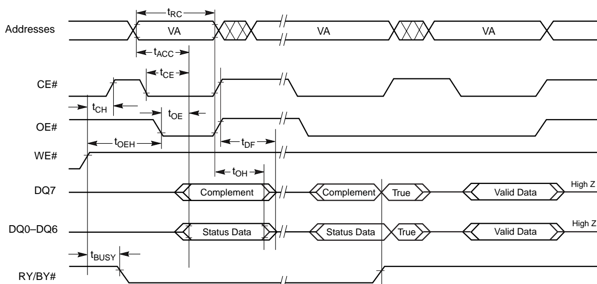
Figure 17. Data# Polling Timings (During Embedded Algorithms)
