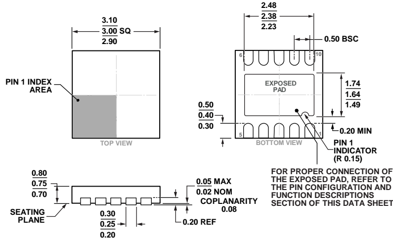
Figure 64. 10-Lead Lead Frame Chip Scale Package [LFCSPP] 3 mm x 3 mm Body and 0.75 mm Package Height (CP-10-9) Dimensions shown in millimeters
