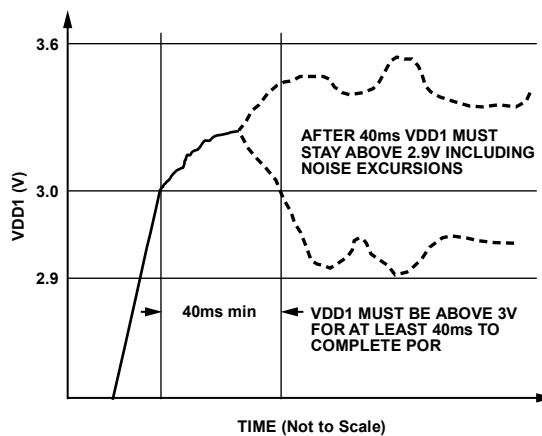
Figure 12. VDD1 Power-On Requirements
