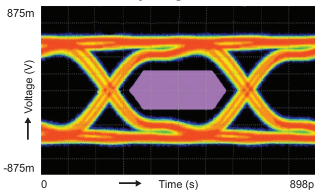
HDMI 1.4 Eye Diagram with AOZ8808
