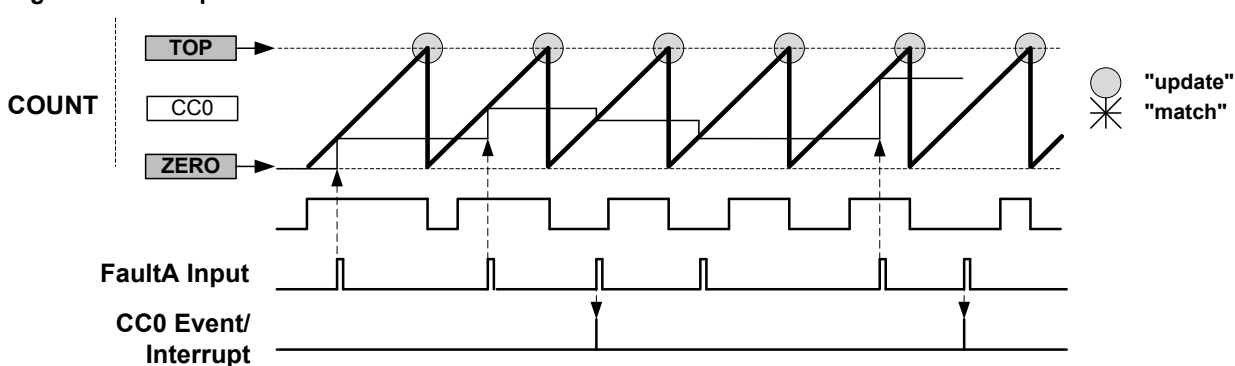
Figure 37-29. Capture Action "DERIV0"
