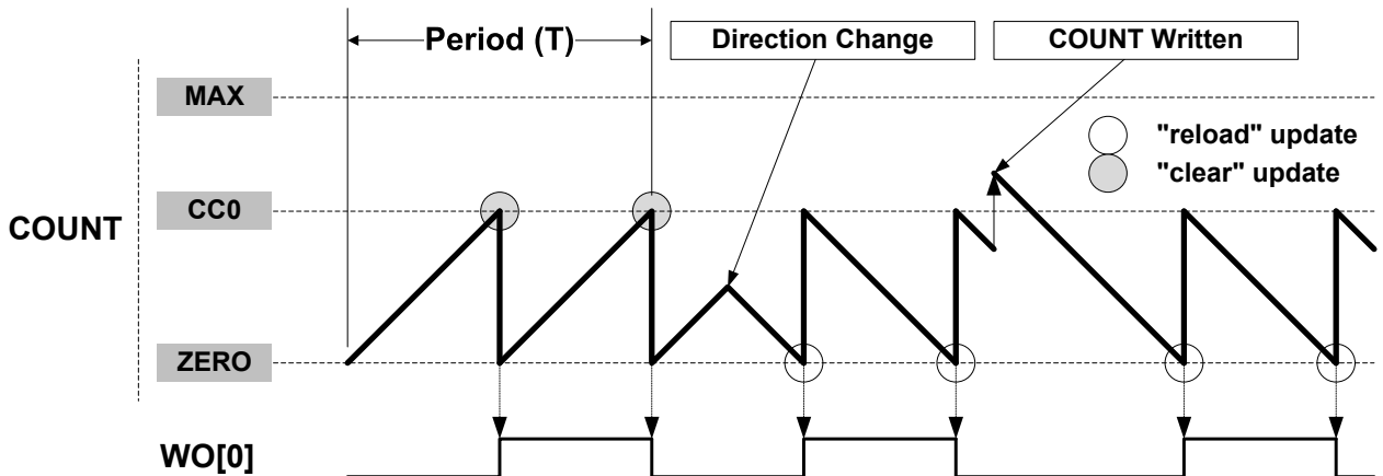
Figure 37-5. Match Frequency Operation
