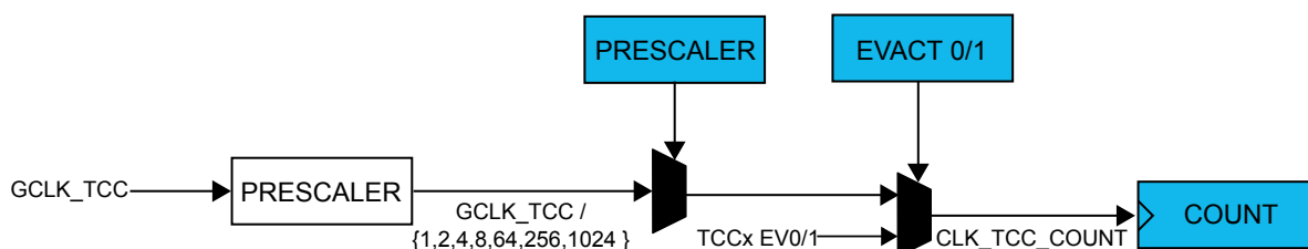
Figure 37-2. Prescaler
