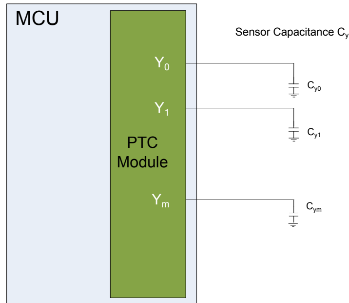
Figure 43-4. Self-capacitance Sensor Arrangement
