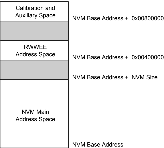
Figure 28-3. NVM Memory Organization
