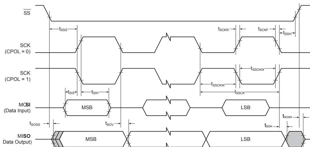
Figure 46-8. SPI Timing Requirements in Slave Mode
