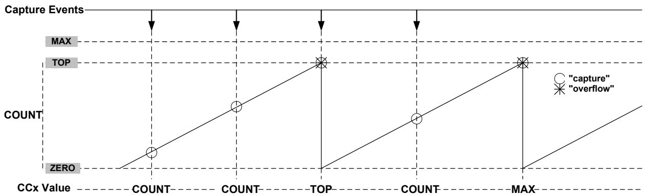
Figure 37-33. Time-Stamp
