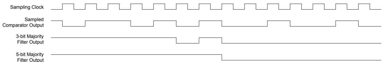
Figure 41-8. Single-Shot Filtering
