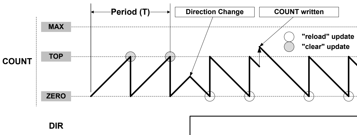
Figure 36-3. Counter Operation
