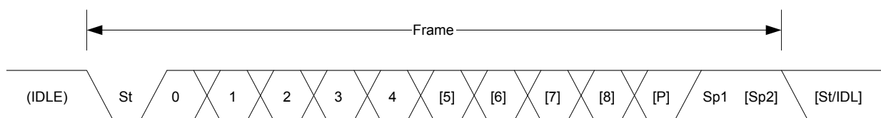
Figure 32-2. Frame Formats
