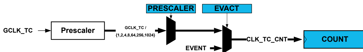
Figure 36-2. Prescaler
