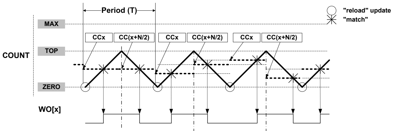
Figure 37-8. Dual-Slope Critical Pulse Width Modulation ( N=\text{CC\_NUM} )
