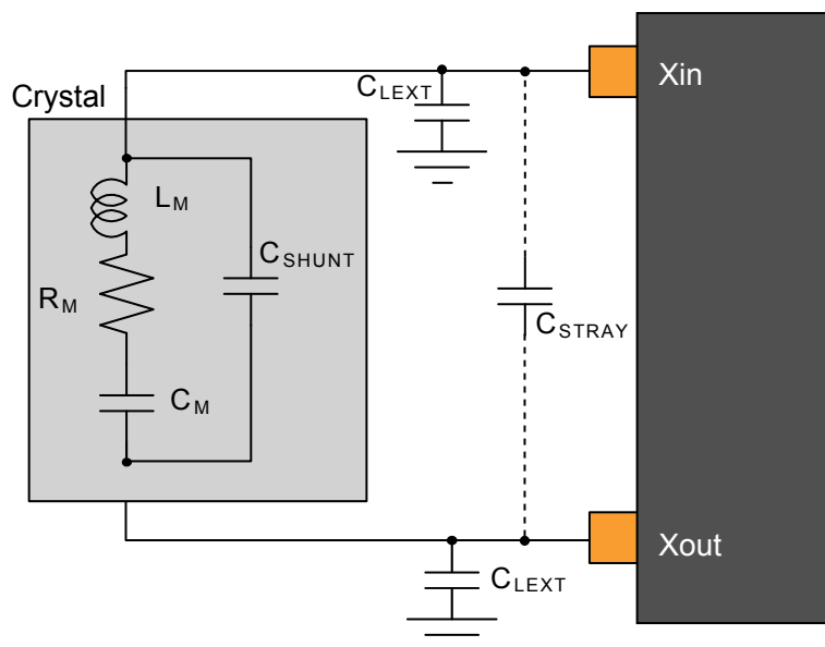
Figure 46-5. Oscillator Connection
