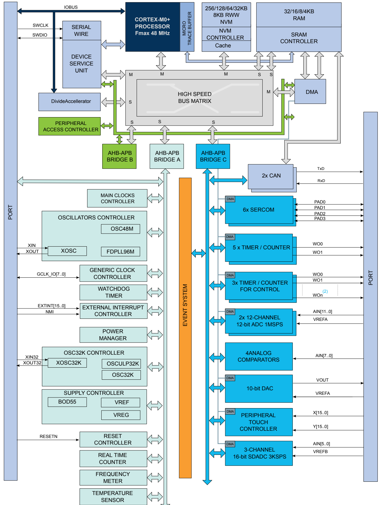
Figure 4-1. System Block Diagram for SAM C21E/G/J
