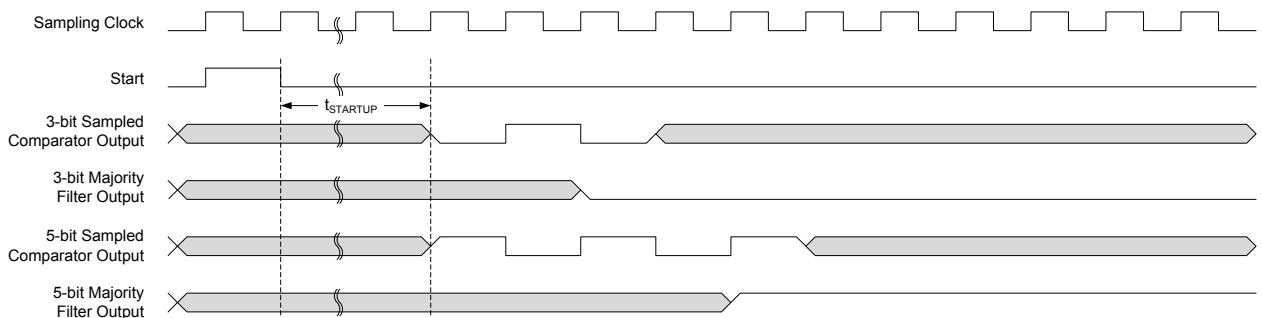
Figure 41-8. Single-Shot Filtering
