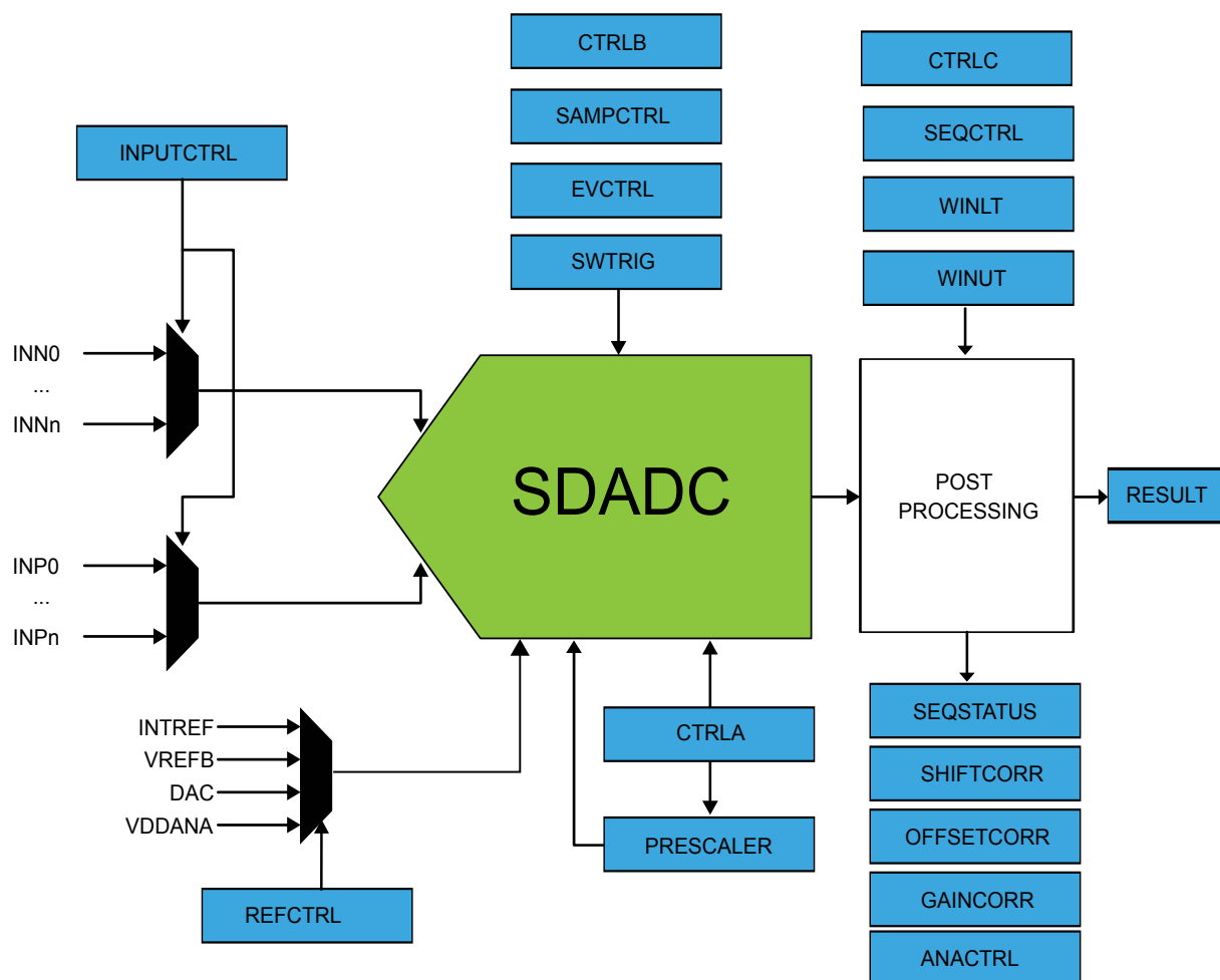
Figure 40-1. SDADC Block Diagram.
