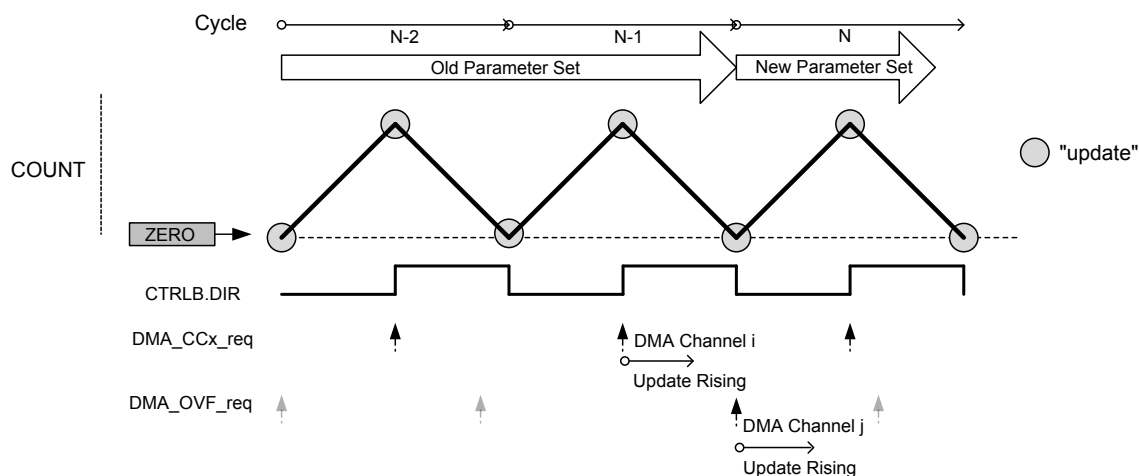
Figure 37-39. DMA Triggers in DSBOTH Operation Mode and Circular Buffer Enabled
