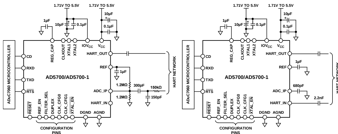
Figure 30. AD5700/AD5700-1 Typical Connection Diagram for External and Internal Filter Options
