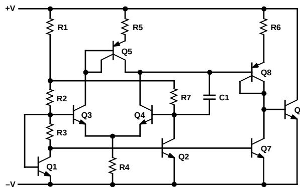
Figure 4. Schematic Diagram
