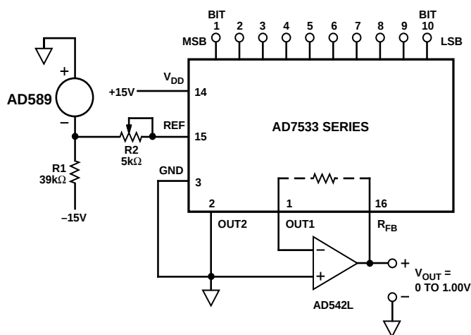
Figure 8. AD589 as Reference for 10-Bit CMOS DAC
