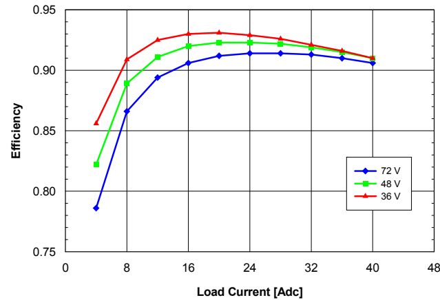
Fig. 3.3V.3: Efficiency vs. load current and input voltage for QME48T40033 converter mounted horizontally with air flowing from pin 1 to pin 3 at a rate of 300 LFM (1.5 m/s) and T_a = 25^{\circ}\text{C} .
