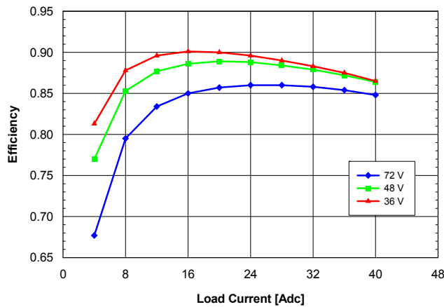
Fig. 1.8V.3: Efficiency vs. load current and input voltage for QME48T40018 converter mounted horizontally with air flowing from pin 1 to pin 3 at a rate of 300 LFM (1.5 m/s) and T_a = 25\text{ }^{\circ}\text{C} .
