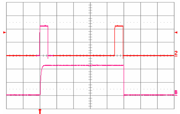
Fig. 1.0V.16: Load current (top trace, 20 A/div., 50 ms/div.) into a 10 m \Omega short circuit during restart, at V_{in} = 48 V. Bottom trace (20 A/div., 5 ms/div.) is an expansion of the on-time portion of the top trace.
