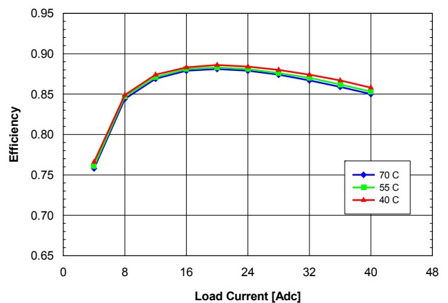
Fig. 1.8V.4: Efficiency vs. load current and ambient temperature for QME48T40018 converter mounted horizontally with V_{in} = 48\text{ V} and air flowing from pin 1 to pin 3 at a rate of 200 LFM (1.0 m/s).
