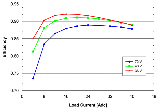
Fig. 2.5V.3: Efficiency vs. load current and input voltage for QME48T40025 converter mounted horizontally with air flowing from pin 1 to pin 3 at a rate of 300 LFM (1.5 m/s) and T_a = 25 °C.
