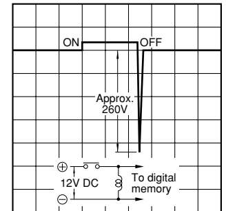
4-(1). DC coil surge voltage waveform (Without diode)
