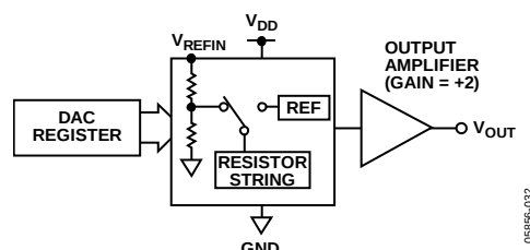
Figure 51. DAC Architecture
