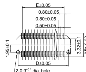
Recommended PC board pattern (TOP VIEW)
