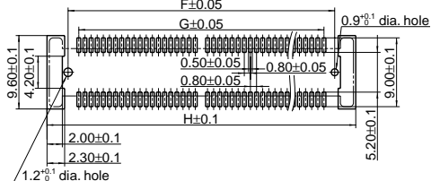
Recommended PC board pattern (TOP VIEW)
