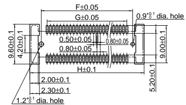
Recommended PC board pattern (TOP VIEW)
