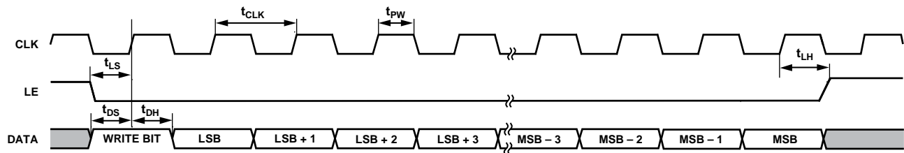
Figure 2. Write Mode Timing Diagram
