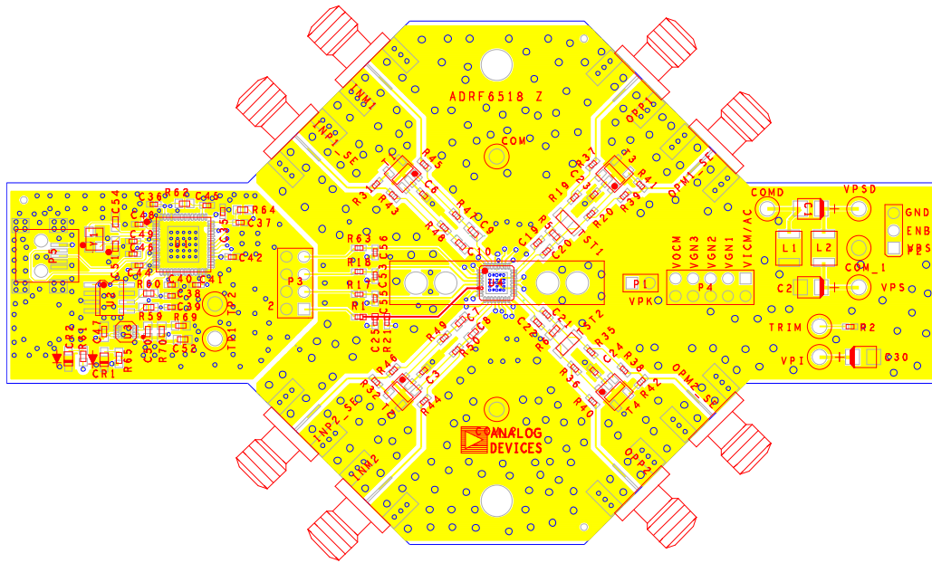
Figure 90. Top Layer Silkscreen
