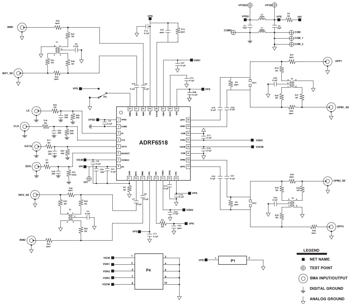
Figure 88. Evaluation Board Schematic
