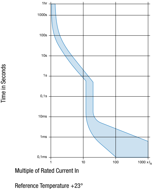
Version H / Magnetic 12-20 xI n
