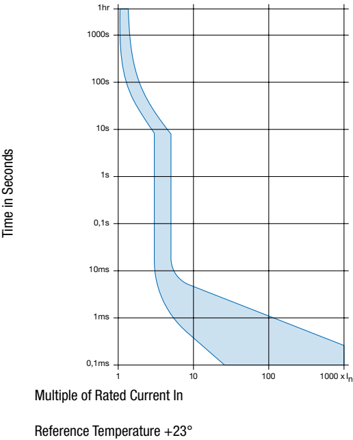
Version F / Magnetic 3-5 xI n
