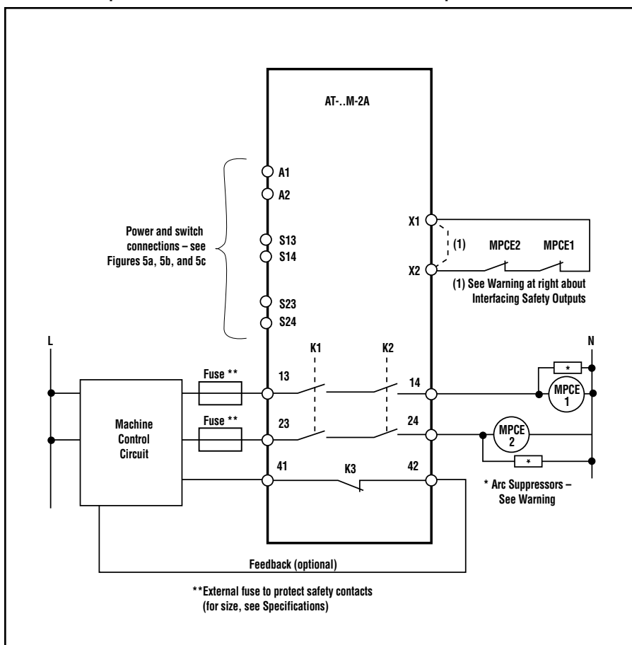
Figure 5d. Machine control circuit connections
