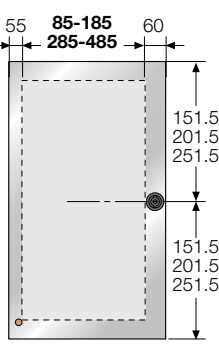
Doors H=300-400-500
