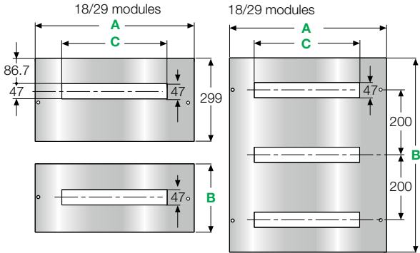
Panels for modular intruments
