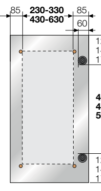
Doors H=600-700-800
