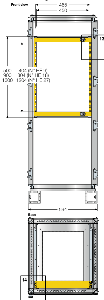
Maximum overall apparatus installation dimensions in 19" swing rack frames
