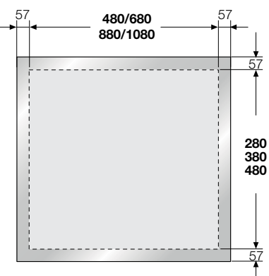
Roof
