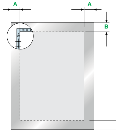
Door/Rear panel
