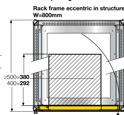
Swing rack frame with 150° opening
