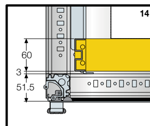
Maximum overall apparatus installation dimensions in 19" swing rack frames
