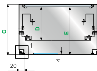
Modular panels and inner door
