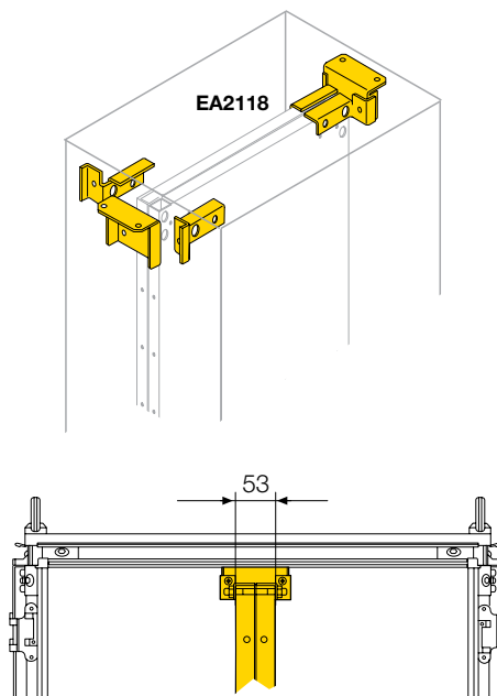
Kit back to back
