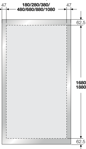
Doors L ≤ 500mm / panels
