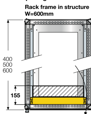
Swing rack frame with 90° opening
