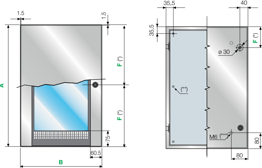
Modular panels and inner door
