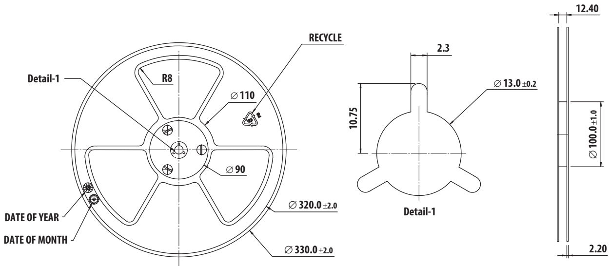
Figure 15. Reel dimensions
