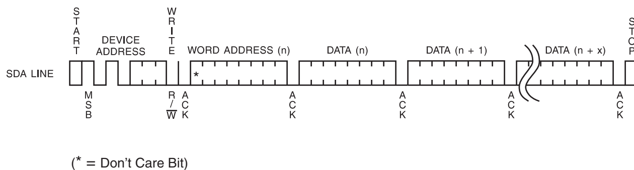
Figure 8-3. Page Write
