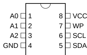
8-Pin PDIP
