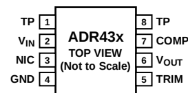
Figure 1. 8-Lead MSOP (RM-8)
