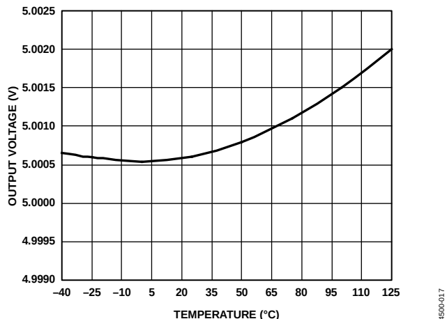
Figure 5. ADR435 Output Voltage vs. Temperature
