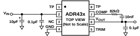
Figure 32. Compensated Reference
