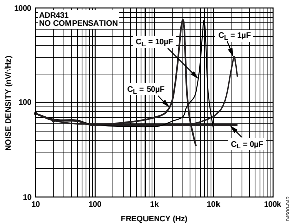
Figure 31. Noise vs. Capacitive Loading
