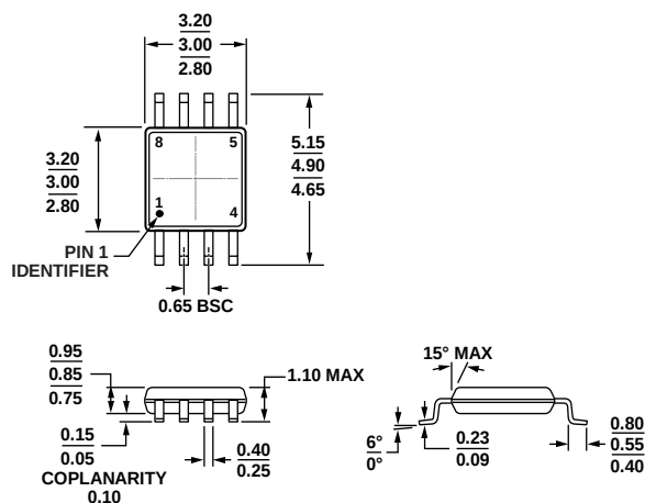
Figure 44. 8-Lead Mini Small Outline Package [MSOP]
