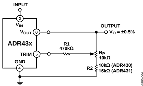
Figure 34. Output Trim Adjustment
