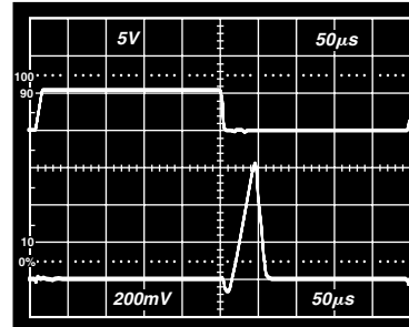
Figure 13. Line Transient Response
