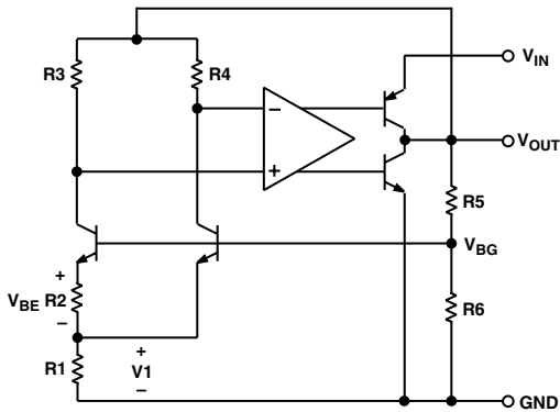
Figure 2. Simplified Schematic
