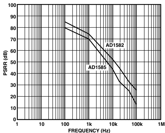
Figure 9b. Ripple Rejection vs. Frequency
