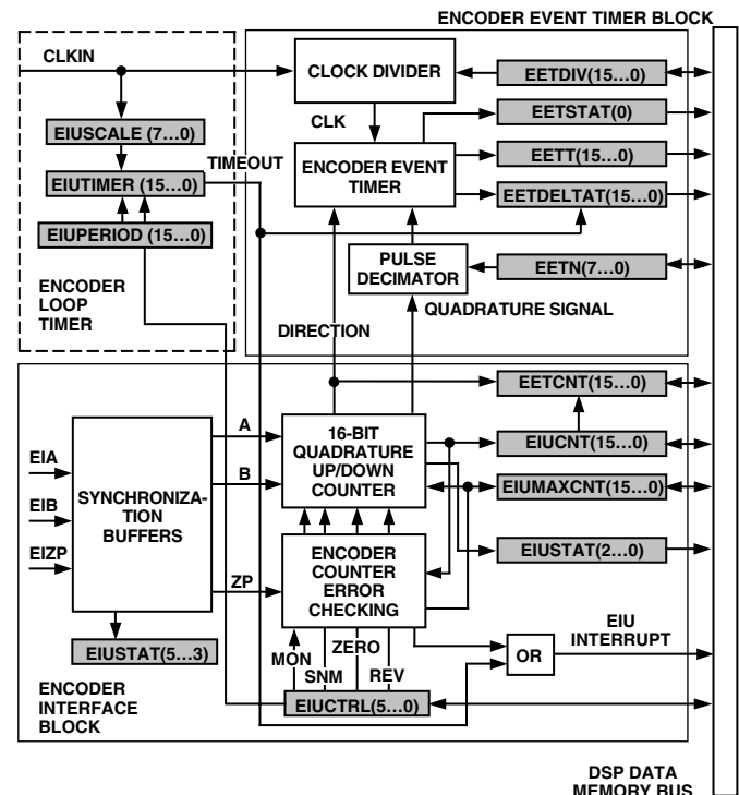
Figure 16. Configuration of Encoder Interface System of ADCM300
