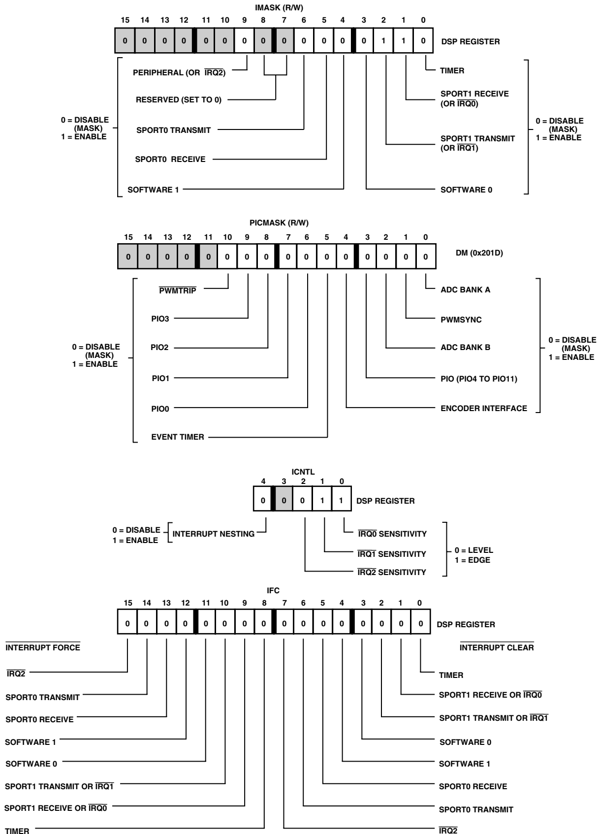
Figure 27. Configuration of ADCM300 Registers
