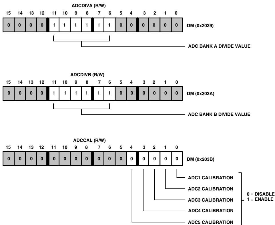
Figure 21. Configuration of ADMC300 Registers
