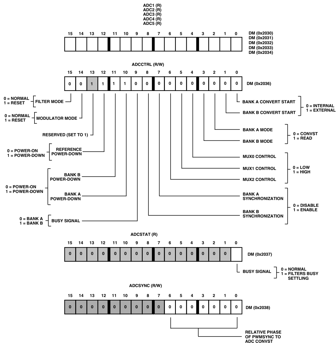
Figure 20. Configuration of ADCM300 Registers
