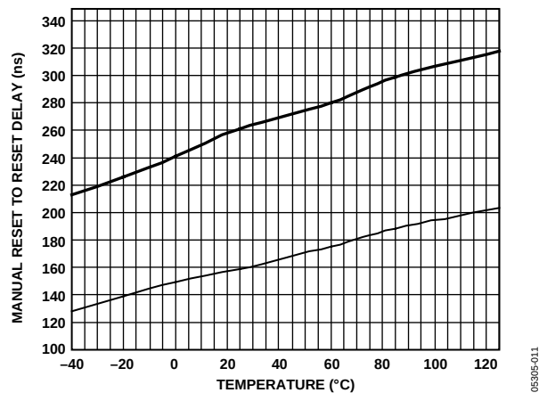
Figure 11. Manual Reset Minimum Pulse Width vs. Temperature
