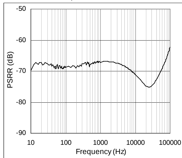
Figure 10. PSRR vs. Frequency; I_{OUT} = 10mA , C_{IN} = 68nF
