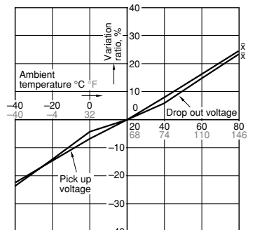
1-(3) Ambient temperature characteristics Sample: AEP51012, 3pcs
