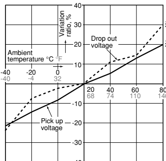
1-(2) Ambient temperature characteristics Sample: AEP16012, 3pcs
