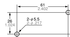
Mounting dimension
