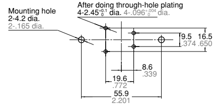
Mounting dimensions
