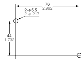
Mounting dimensions
