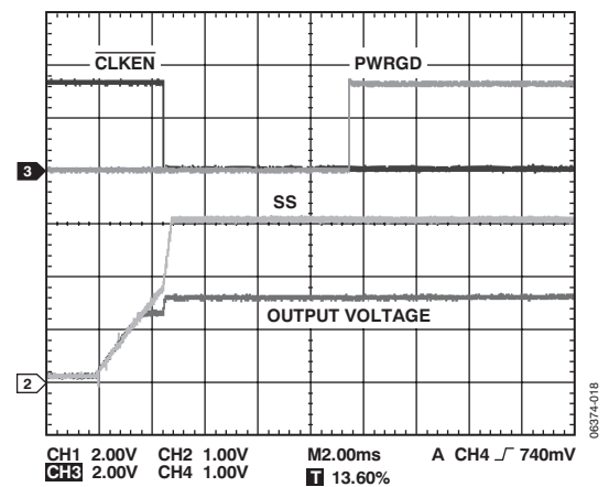
Figure 18. Start-Up Waveforms
