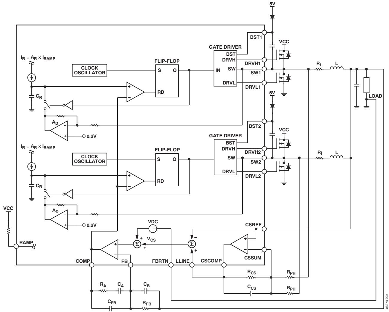
Figure 25. Dual-Phase PWM Mode Operation
