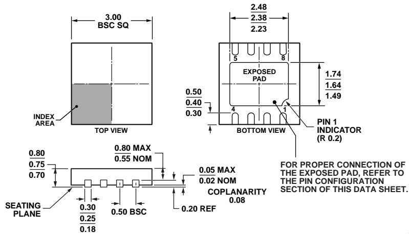
Figure 58. 8-Lead Lead Frame Chip Scale Package [LFCSWP_WD] 3 mm x 3 mm Body, Very Very Thin, Dual Lead (CP-8-5)
