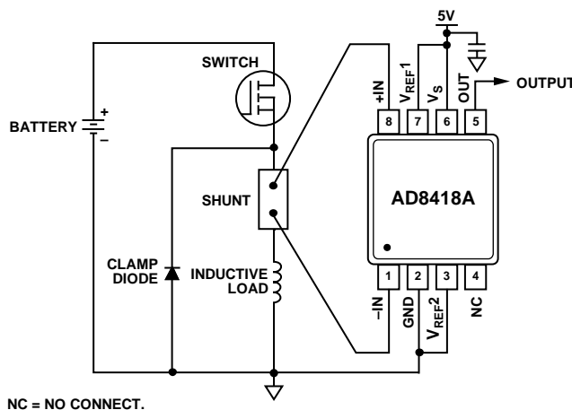
Figure 35. High-Side Switch
