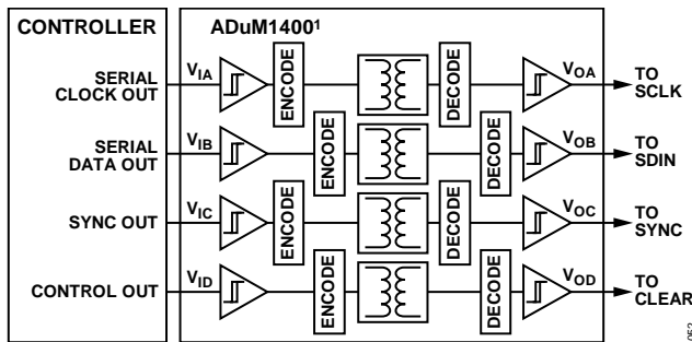
Figure 58. Isolated Interface
