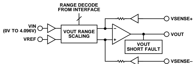
Figure 54. Voltage Output
