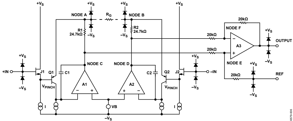
Figure 55. Simplified Schematic
