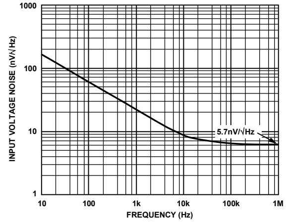
Figure 38. Voltage Noise (RTI)
