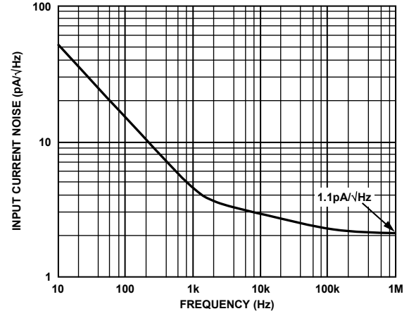
Figure 37. Current Noise (RTI)
