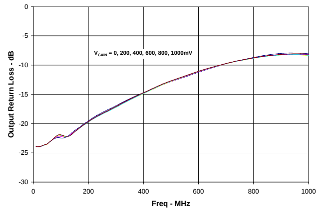
Figure 7. Output Return Loss vs. Frequency
