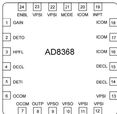
Figure 2. 24-Lead LFCSP
