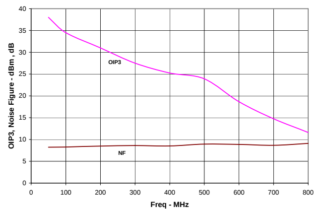
Figure 7. OIP3 and NF vs. Frequency
