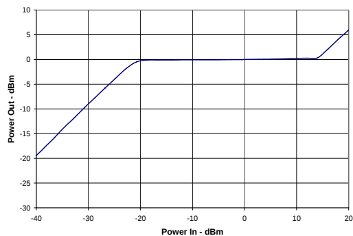
Figure 13 Output Power versus Input Power in AGC Mode at 140MHz.
