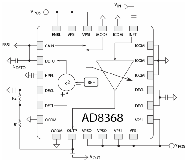
Figure 12. AGC Mode of Operation
