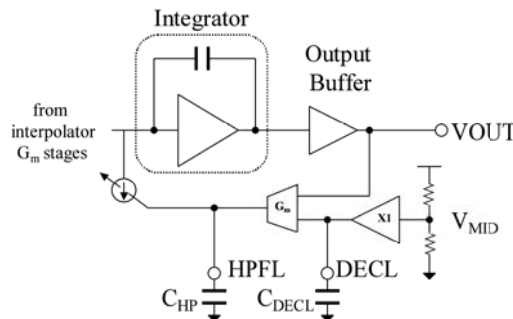
Figure 9. Output Centering Control Loop
