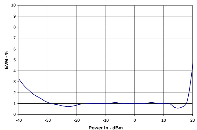
Figure 15. Error Vector Magnitude Performance for 16-QAM 10MSymbols/sec.
