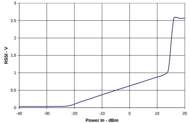
Figure 14. Monitoring the GAIN/DETO RSSI Voltage versus Input Power.
