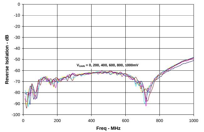
Figure 6. Reverse Isolation vs. Frequency
