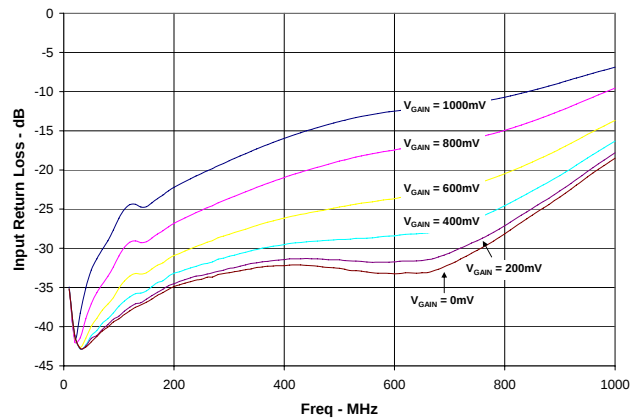
Figure 4. Input Return Loss vs. Frequency
