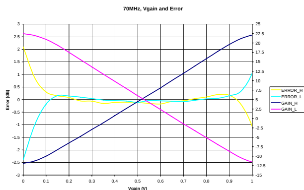
Figure 10 The gain function can be either an increasing or decreasing function of VGAIN, depending on the MODE pin.
