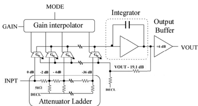
Figure 8. Simplified Block Diagram
