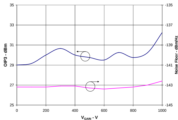
Figure 5. OIP3 and Output Noise Floor vs. V_{GAIN} at 140MHz
