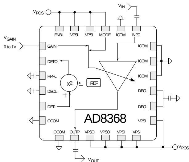
Figure 11. Typical Connections for VGA Mode
