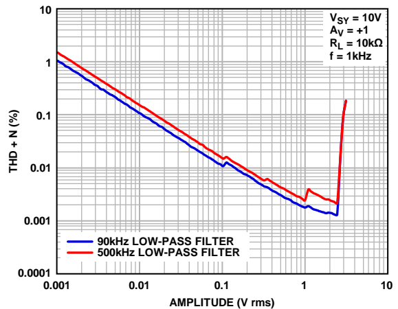
Figure 83. THD + N vs. Amplitude, V_{SY} = 10\text{ V}
