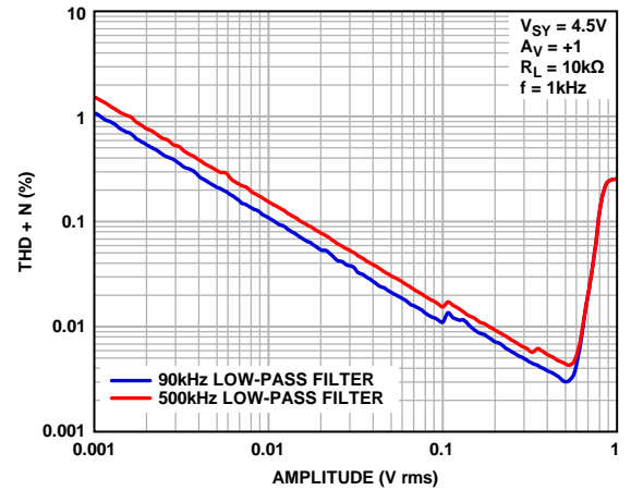
Figure 82. THD + N vs. Amplitude, V_{SY} = 4.5\text{ V}
