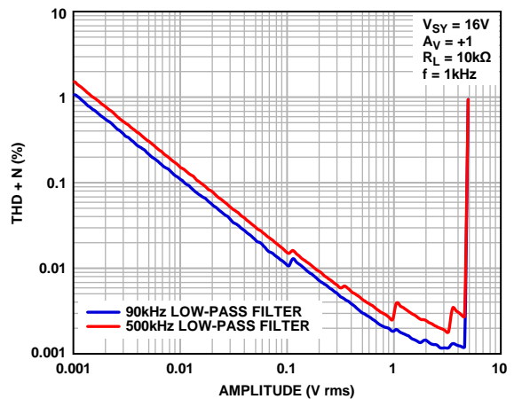
Figure 84. THD + N vs. Amplitude, V_{SY} = 16\text{ V}
