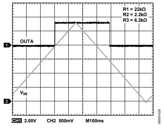
Figure 27. Hysteresis Programmed to ~513 mV at Top of Input String (Hysteresis at ADCMP341 Pins \approx 104 mV)
