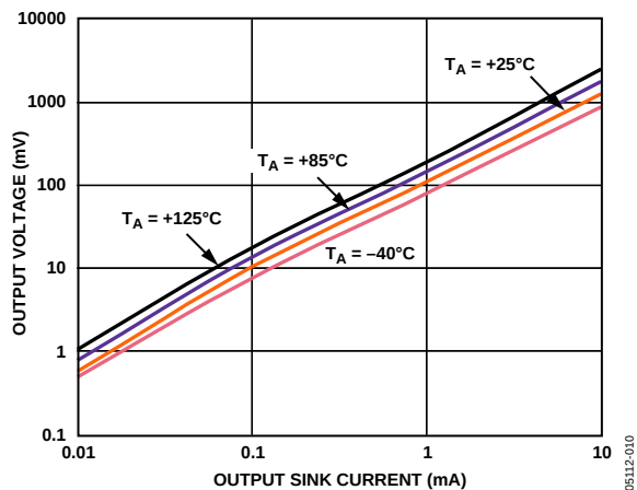
Figure 13. Output Voltage vs. Output Sink Current ( I_{SINK} = 500\text{ mA} )
