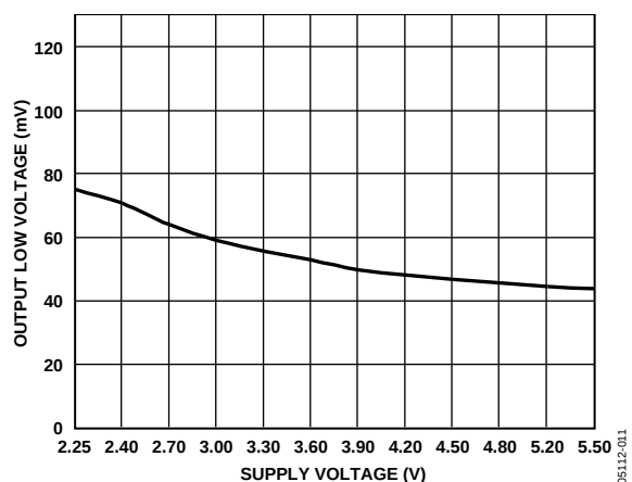
Figure 14. Output Low Voltage vs. Supply Voltage ( I_{SINK} = 500\text{ mA} )
