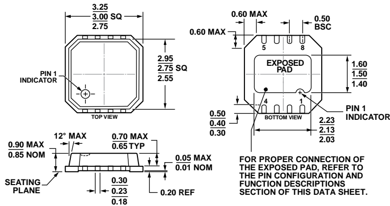
Figure 43. 8-Lead Lead Frame Chip Scale Package [LFCSP_VD] 3 mm × 3 mm Body, Very Thin, Dual Lead (CP-8-9) Dimensions shown in millimeters
