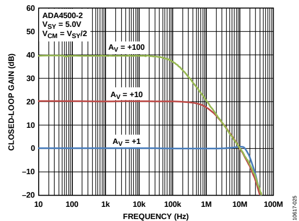
Figure 28. Closed-Loop Gain vs. Frequency, V_{SY} = 5.0\text{ V}
