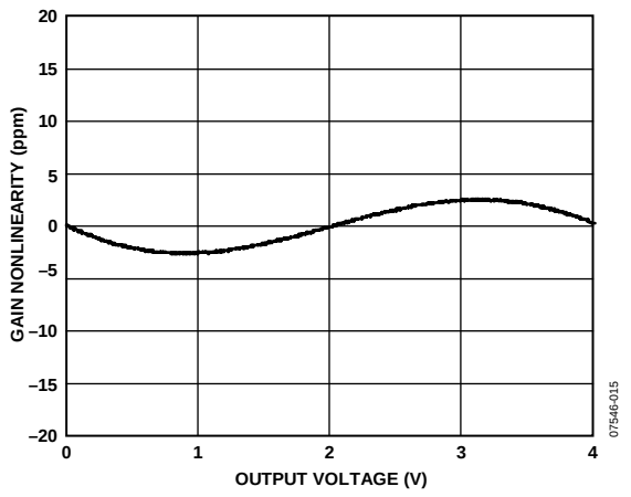
Figure 16. Gain Nonlinearity, R_L = 600\ \Omega , 2\ \text{k}\Omega , 10\ \text{k}\Omega
