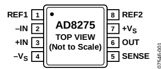
Figure 4. Pin Configuration
