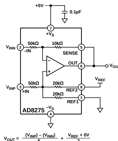
Figure 34. Basic Configuration 2: Split Reference
