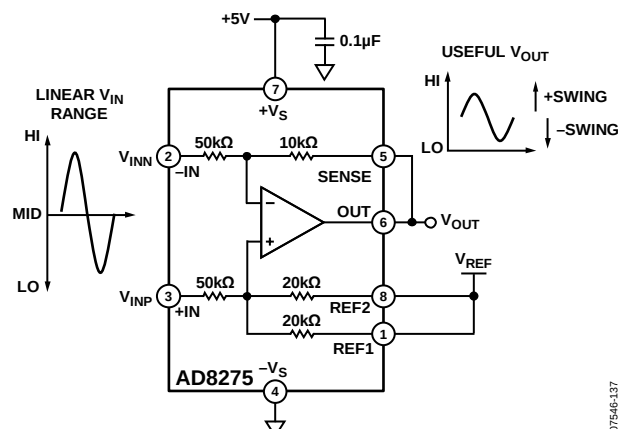
Figure 37. Shared Reference
