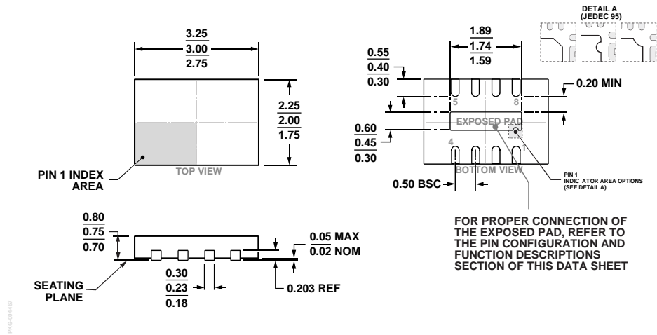
Figure 44. 8-Lead Lead Frame Chip Scale Package [LFCSPP] 2 mm x 3 mm Body and 0.75 mm Package Height (CP-8-23) Dimensions shown in millimeters
