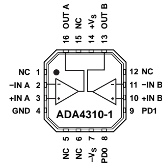
Figure 2. Thermally Enhanced, 4 mm × 4 mm 16-Lead LFCSP_VQ
