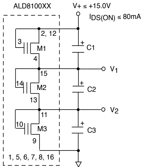
TYPICAL SERIES CONNECTION OF SAB MOSFET WITH THREE SUPERCAPS
