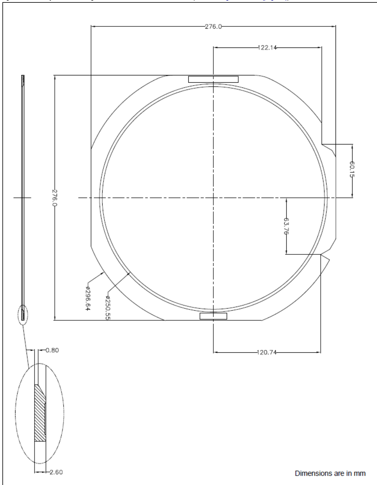
Figure 18. Delivery Frame drawing for '8" cut DfEs on Foil in 12" Frame' (see Ordering Information (page 41) )
