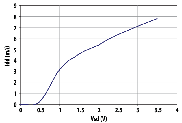
Figure 6. Idd vs Vsd for Vdd = 2.8V, R2 = 3.9k 0hm
