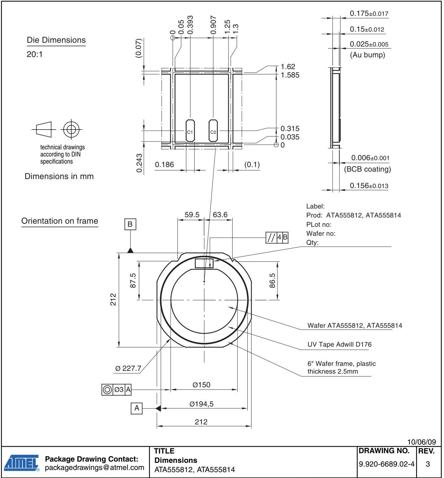
Figure 10-3. 6" Sawn Wafer on Foil with Ring and Goldbumps 25 μm (Type 12/14, Mega Pads)
