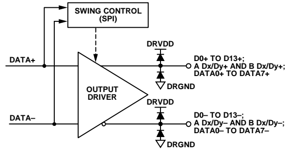
Figure 36. Digital Outputs
