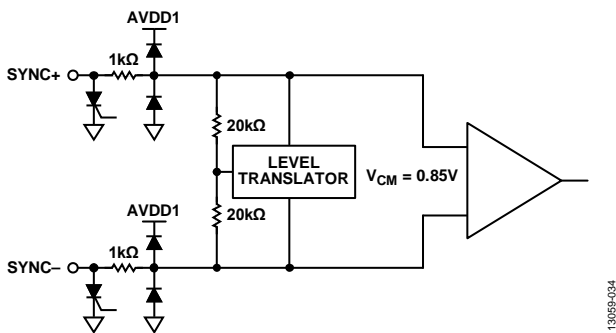
Figure 35. SYNC± Inputs
